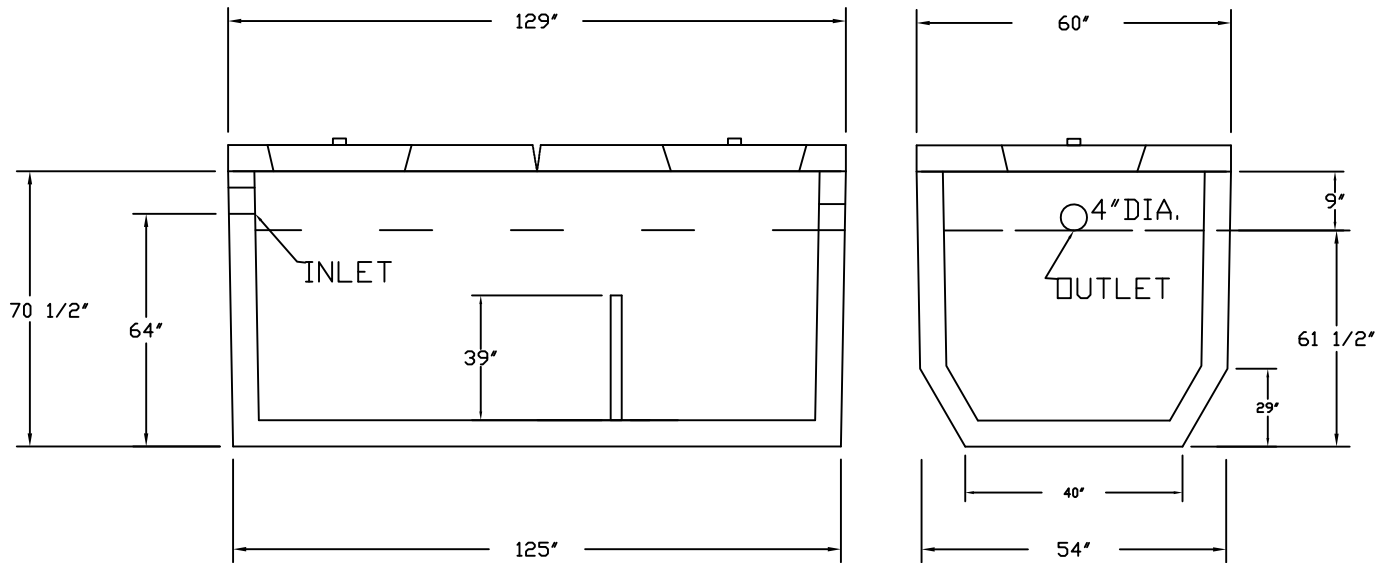
SIDE VIEW
