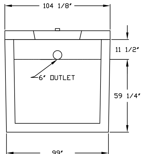
END VIEW
