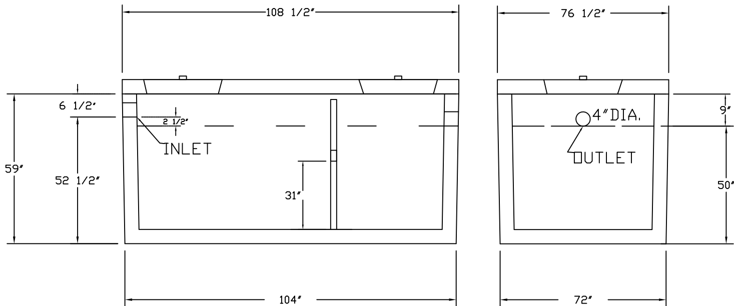
SIDE VIEW
