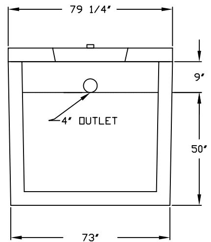
END VIEW
