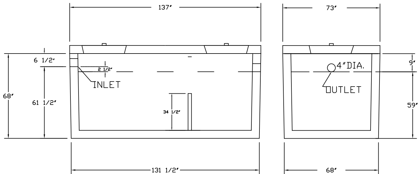
SIDE VIEW
