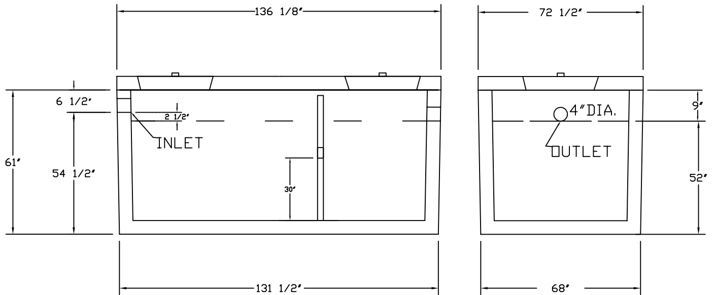
SIDE VIEW
