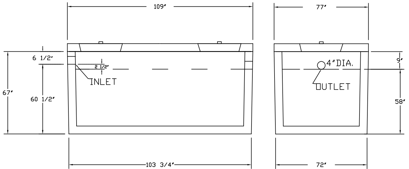
SIDE VIEW
