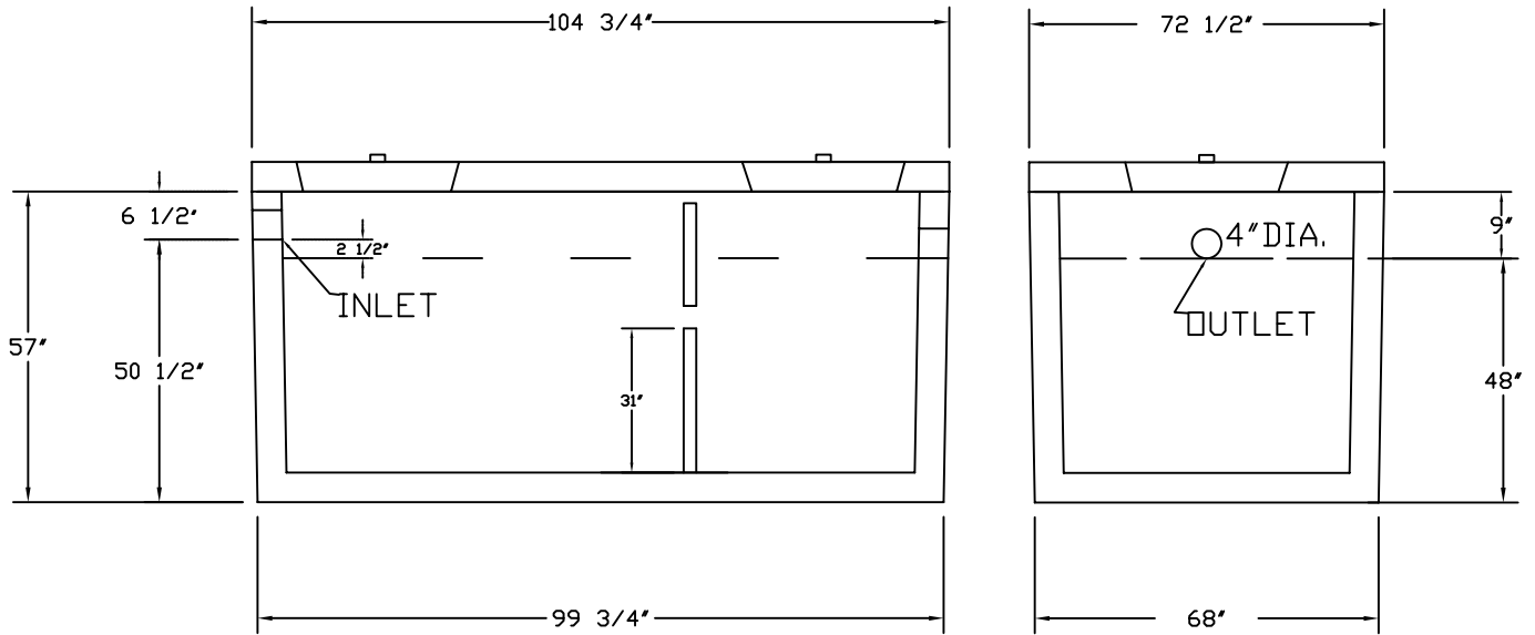
SIDE VIEW
