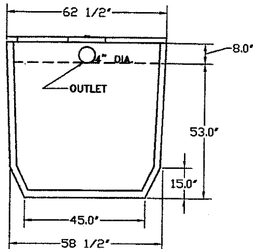
END VIEW
